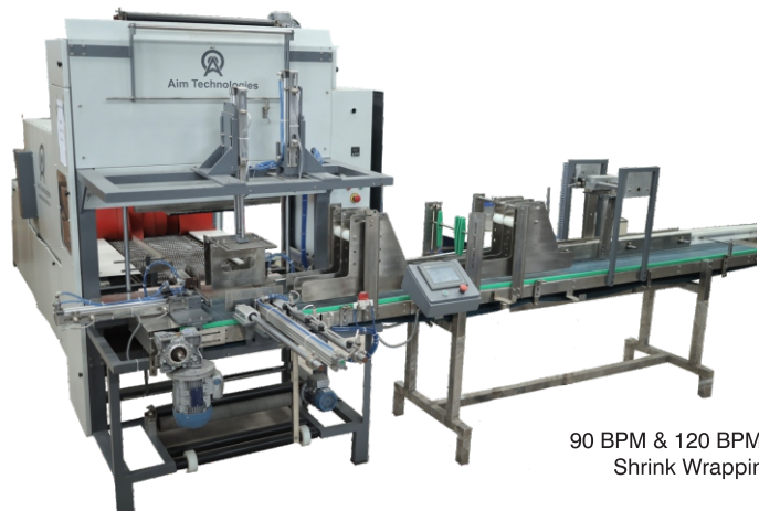
Linear Shrink Wrapping Machine
