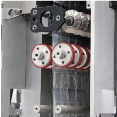
Draw - off rollers for web transportation and longitudinal cutters
